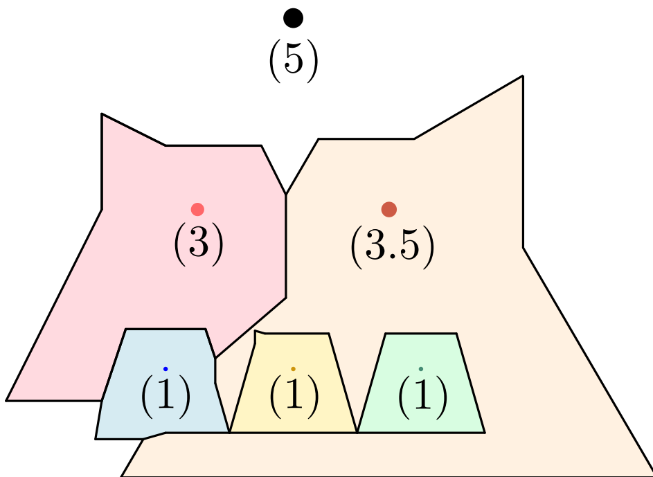
\mathcal{V}^\infty – Example
